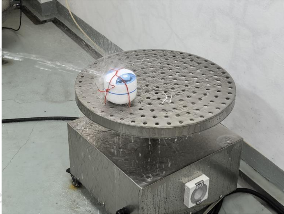
Waterproof test photo (US 202)
