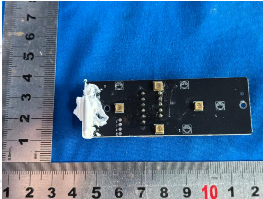
After waterproof test photo (US 202)
